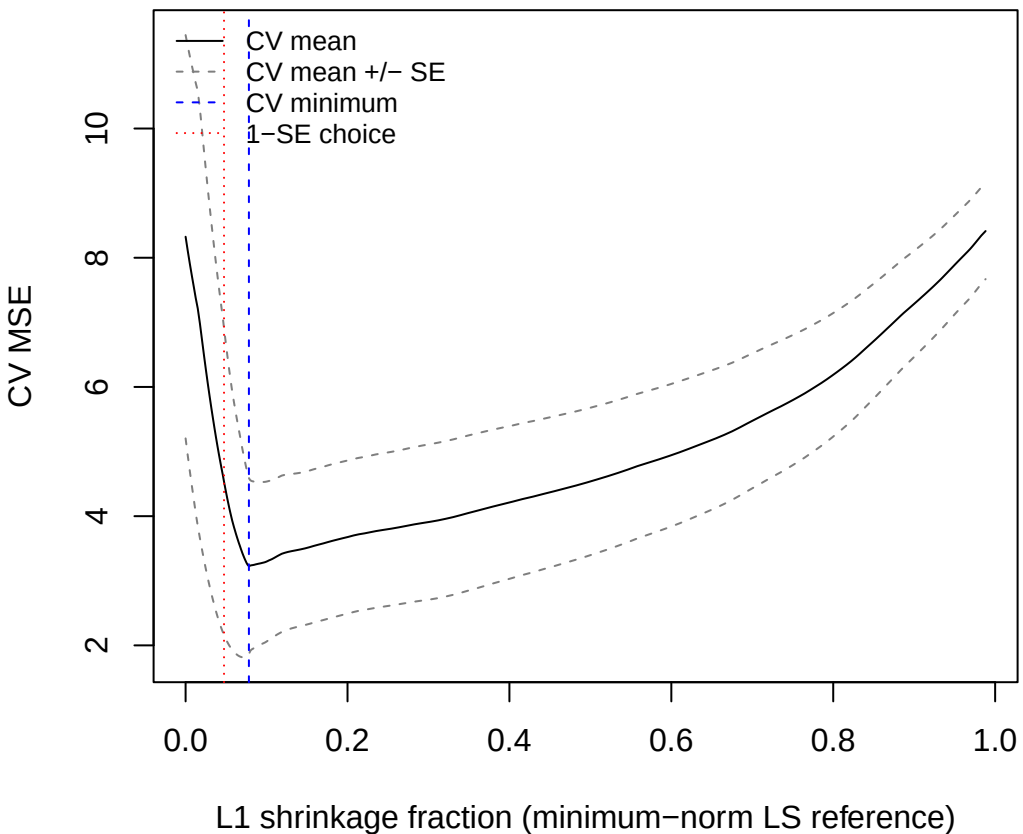
5 fold CV with one-SE bands
