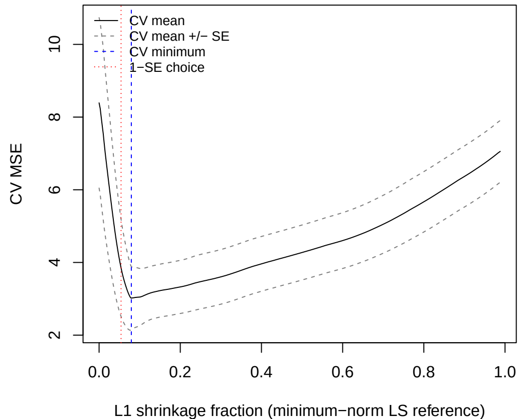
10 fold CV with one-SE bands
